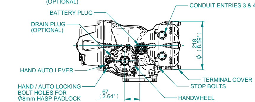
VIEW ON ARROW 'A'
